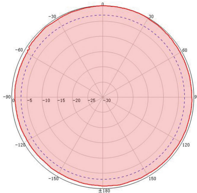
Axial Ratio
